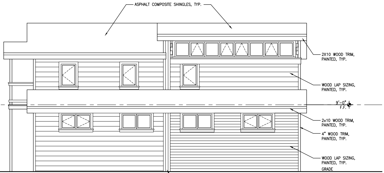
1 SOUTH ELEVATION A3.0 SCALE: 1/8"=1'-0"
