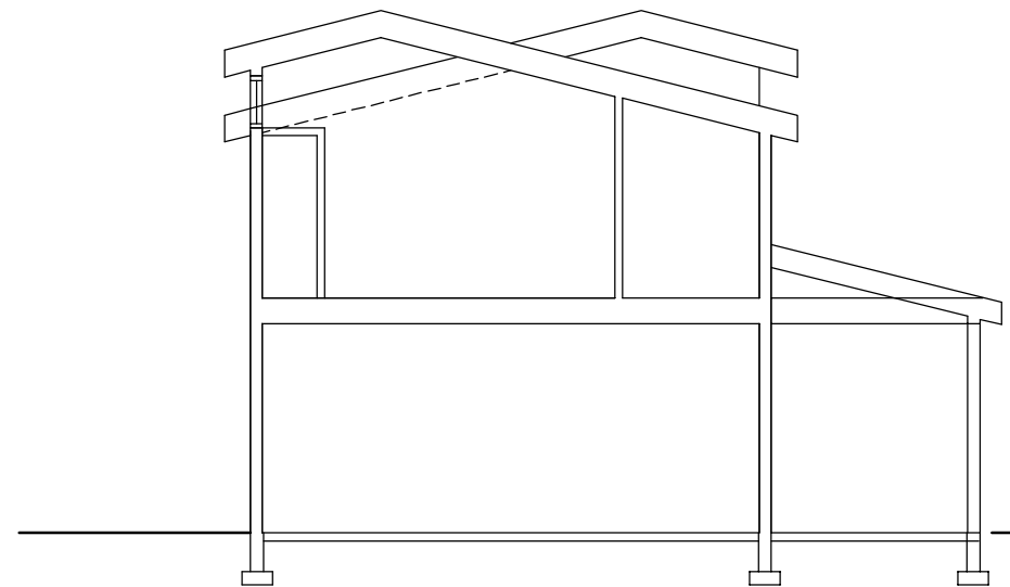
6 BUILDING SECTION A3.0 SCALE: 1/8"=1'-0"
