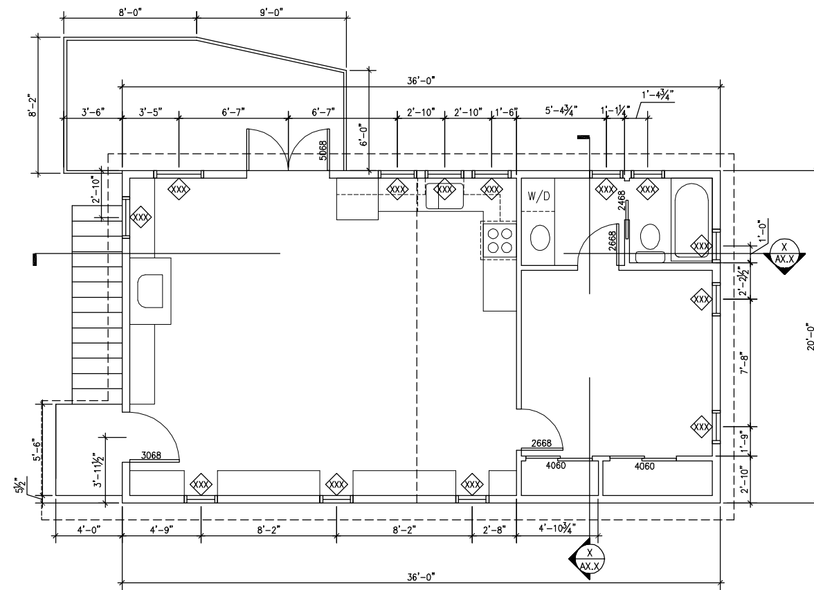
1 SECOND FLOOR PLAN A3.0 SCALE: 1/4"=1'-0"
